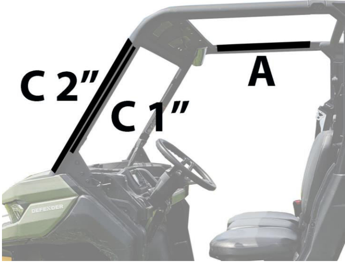
Figure 1: Place adhesive Velcro as shown in photo. 2" strip C is for the Velcro sewn on to the front of the door kit, 1" strip C is for the straps sewn onto the front of the door panel. Wrap straps around the roll bar and attach to 1" strips C.
