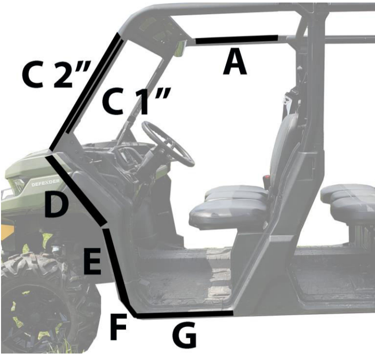
Figure 1: Place adhesive Velcro as shown in photo. 2" strip C is for the Velcro sewn on to the front of the door kit, 1" strip C is for the straps sewn onto the front of the door panel. Wrap straps around the roll bar and attach to 1" strips C.
