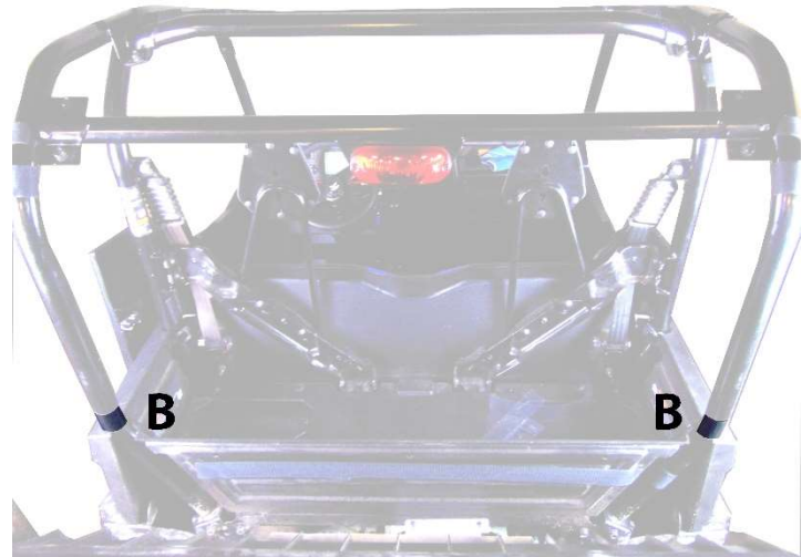
Figure 2: WRAP THESE VELCRO STRIPS AROUND THE ROLL BAR AND ATTACH DOUBLE-SIDED STRAPS.
