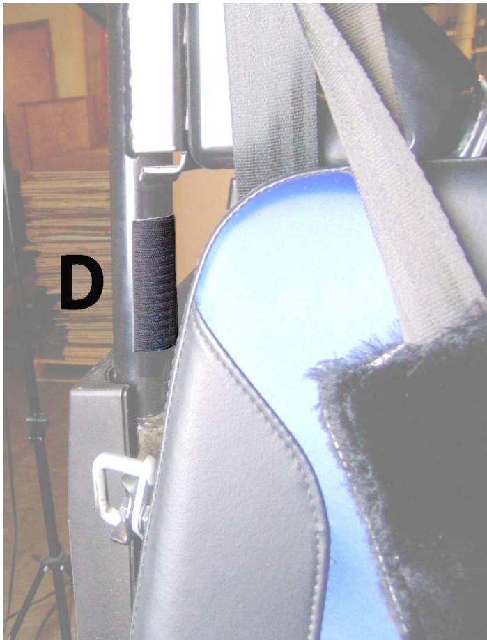
Figure 4: Shows placement of 4" Velcro strip D. You will install a Velcro strips in the same position on the opposite side of the UTV.
