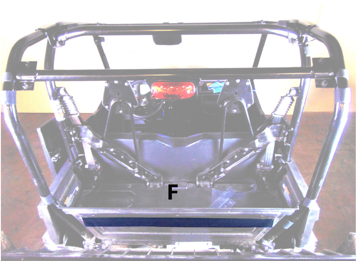
Figure 6: Shows placement of 38" Velcro strip F.
