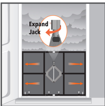
Jack expands and seals sides
