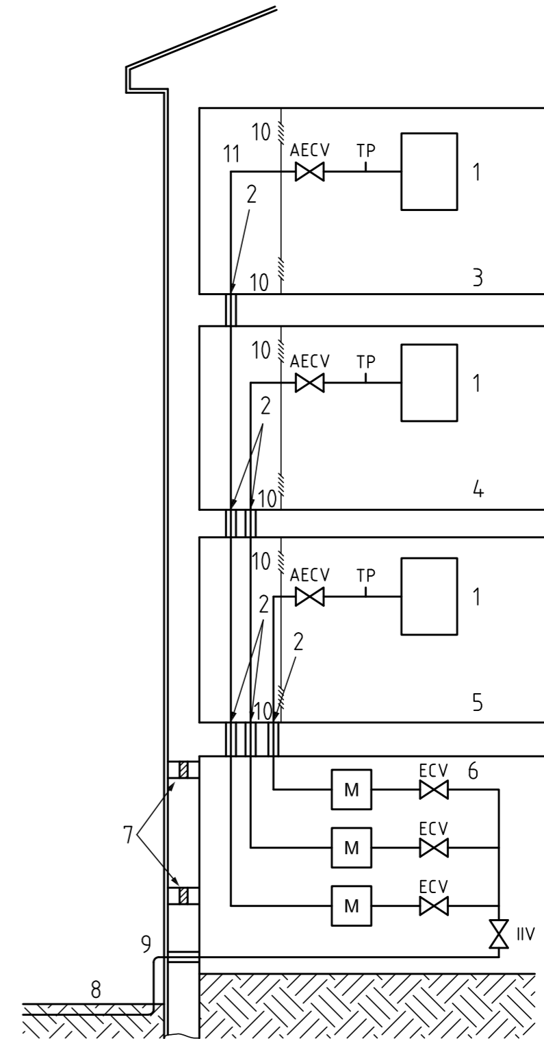
b) Fire stopped pipework and ventilated enclosed area
