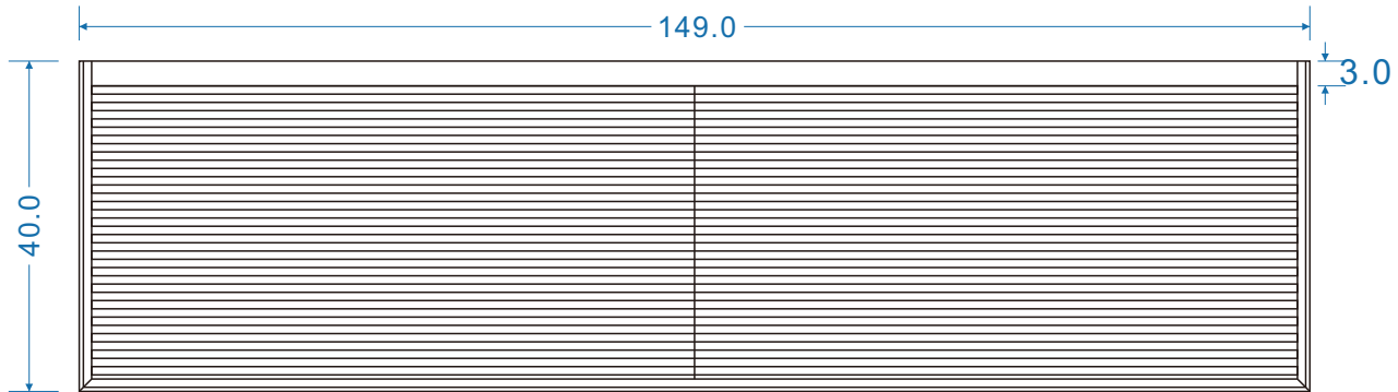
FRONT VIEW
