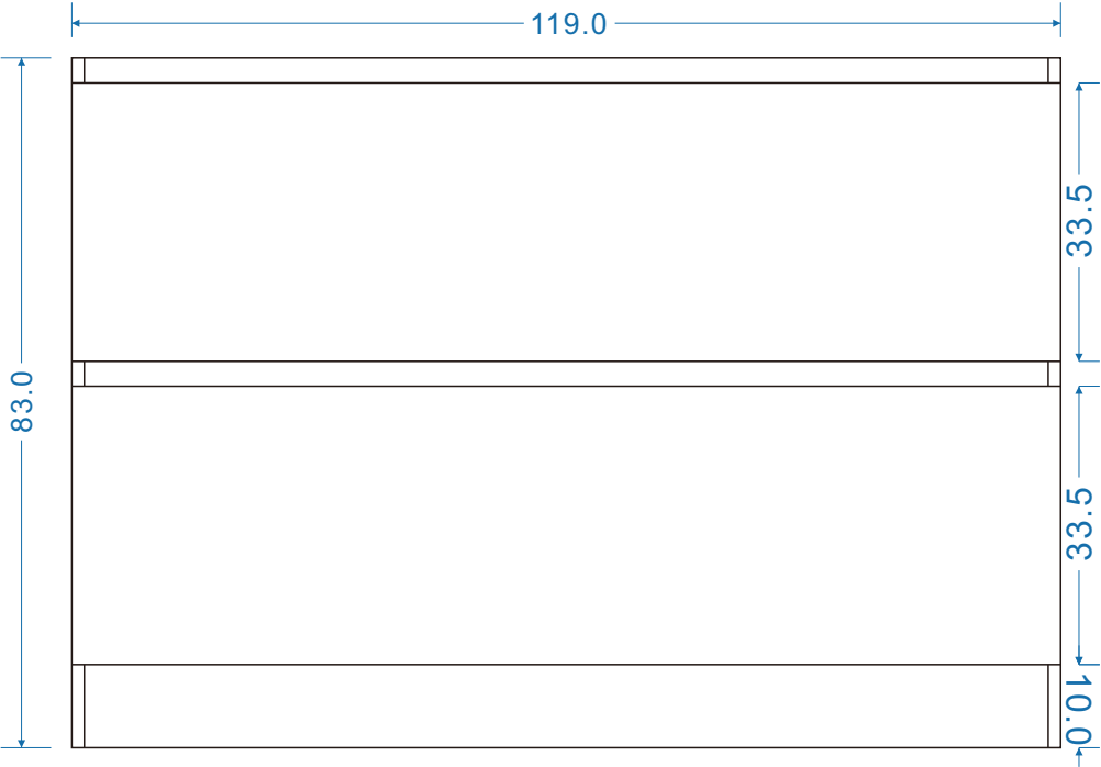
FRONT VIEW
