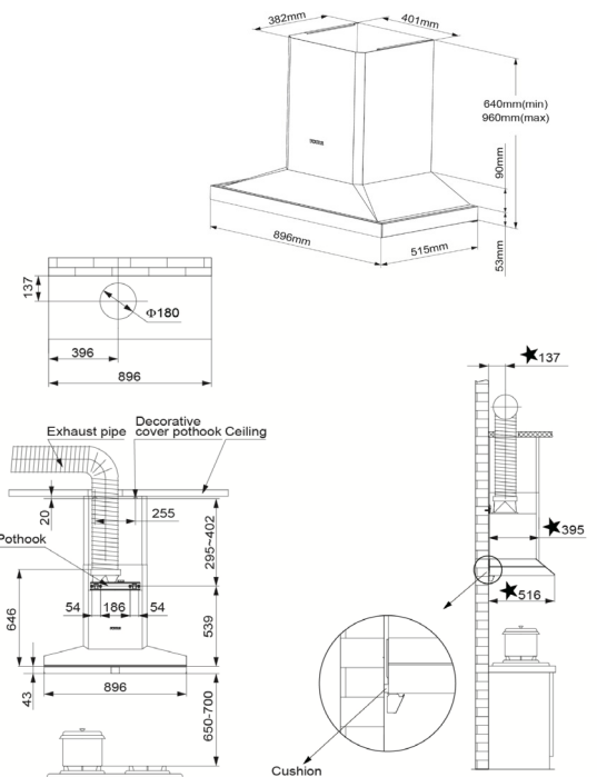
Product installation and cabinet collocation figure diagram (★ is the distance from the wall)
