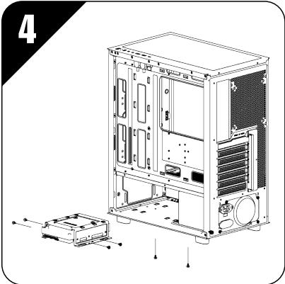
Installing SSD and HDD hard drives
