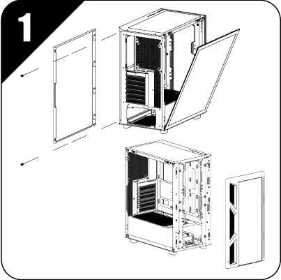
Open the left glass and right iron plate remove the front plate
