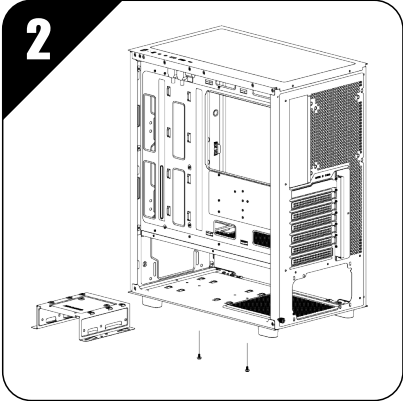
Removing the hard drive rack
