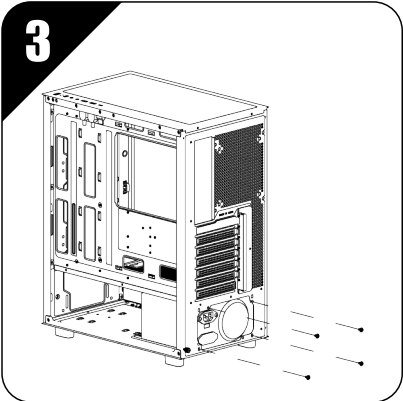
Installing power supply
