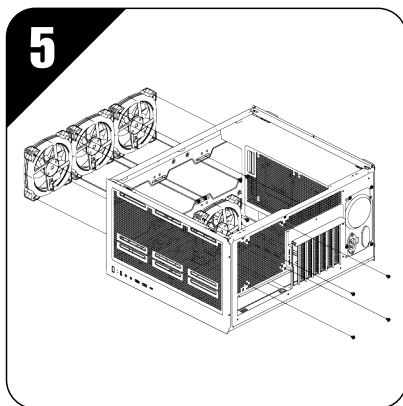
Installing the front panel fan
