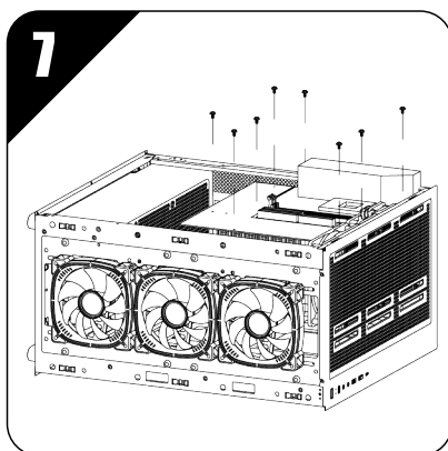
Installing the motherboard
