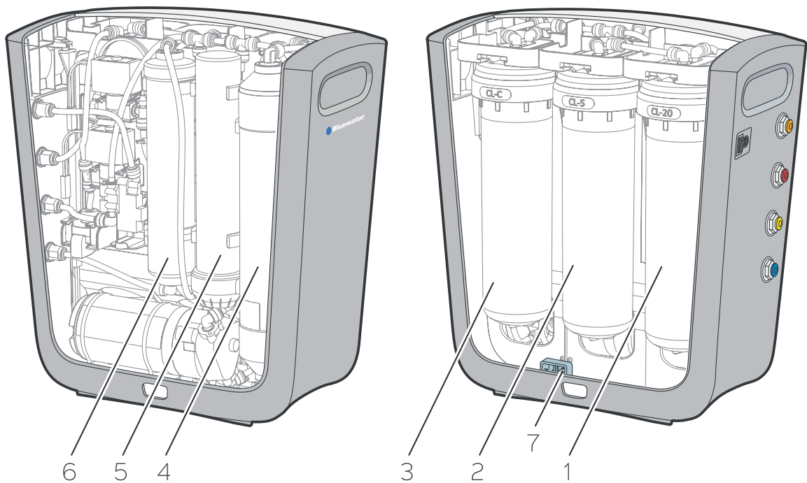
Figure 4. Cleone inside
