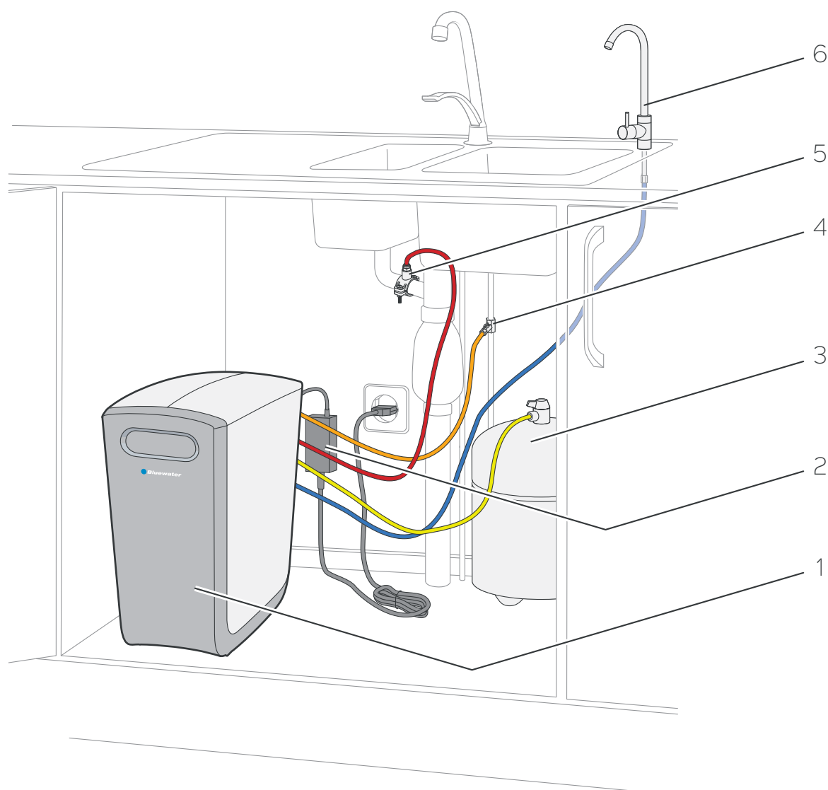
Figure 5. System overview
