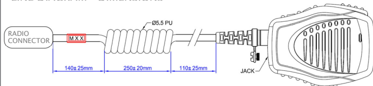
LINE DIAGRAM—DIMENSIONS
