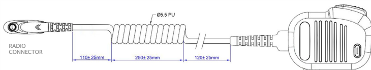
LINE DIAGRAM—DIMENSIONS
