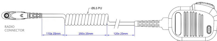
LINE DIAGRAM—DIMENSIONS
