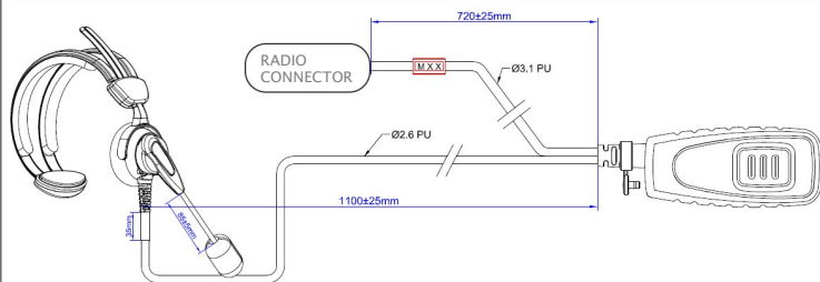
LINE DIAGRAM—DIMENSIONS
