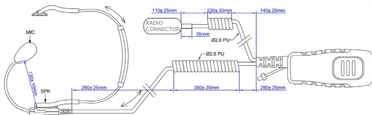
LINE DIAGRAM—DIMENSIONS
