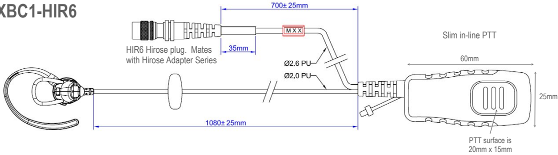
Remote PTT Button Option for XBC1/XBC2
