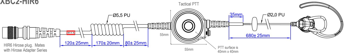
Remote PTT Button Option for XBC1/XBC2
