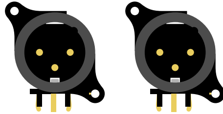
J2, J4 3-pin XLR male
