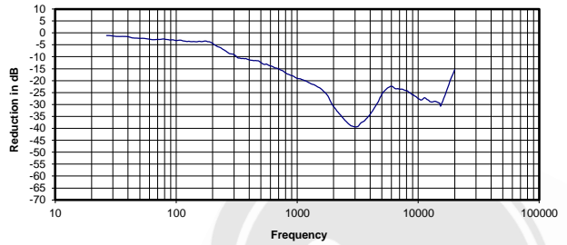
Isolation Attenuation of External Sound vs. Frequency
