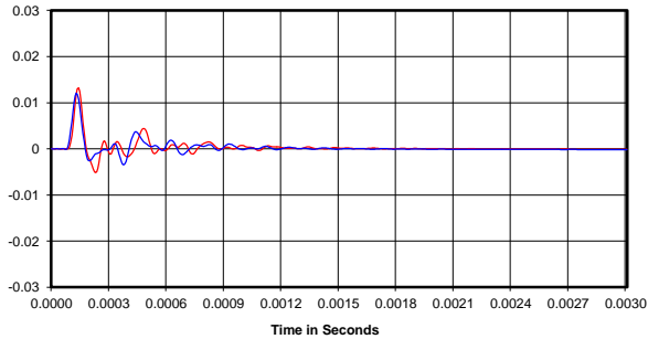
Impulse Response
