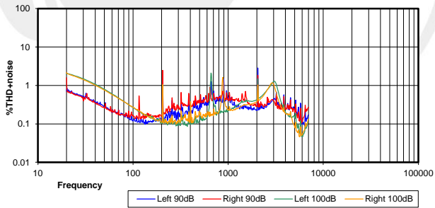
%THD+noise @ 90dB and 100dB
