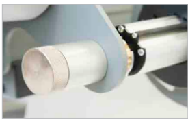
Adjustable unwinding shaft for fine positioning of the material unrolling (optional)
