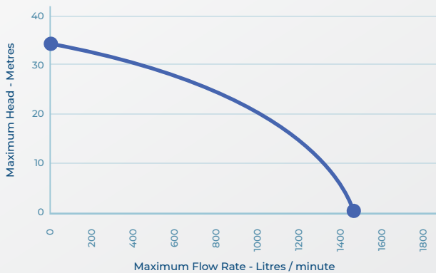
MH40-2 PUMP PERFORMANCE CURVE
