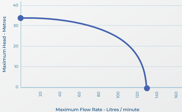
MH10-2 PUMP PERFORMANCE CURVE
