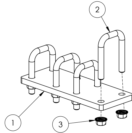
41827 Splice Bracket
