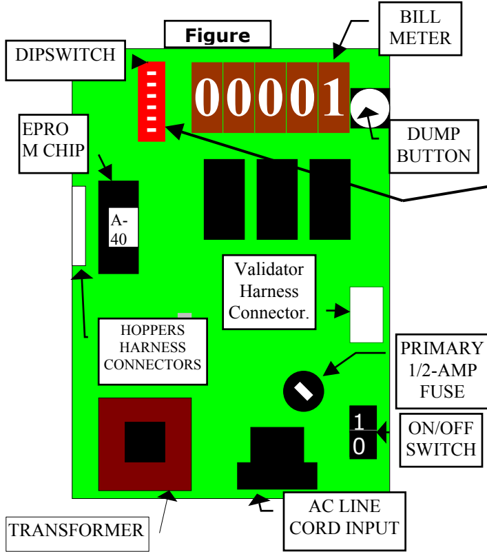
FIGURE 2 (THIS IS NOT THE DIPSWITCH BANK FOR SETTING THE BILL DENOMINATIONS. (For those dip switches go to page 10.)
