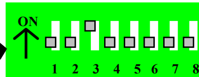
FIGURE 2 (THIS IS NOT THE DIPSWITCH BANK FOR SETTING THE BILL DENOMINATIONS. (For those dip switches go to page 10.)
