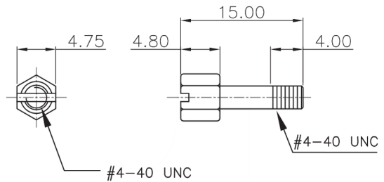
Screw specification
