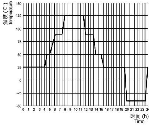
3. 电耐久试验环境温度曲线 Ambient Temperature Curve of the Electrical Endurance Test
