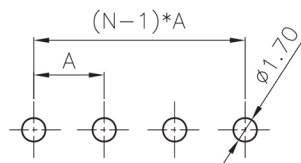
RECOMMEND PCB LAYOUT (TOLERANCE = ± 0.05)
