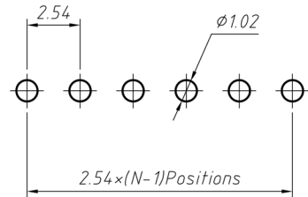
Recommended P.C.B Hole Layout
