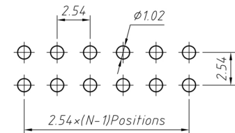
Recommended P.C.B Hole Layout
