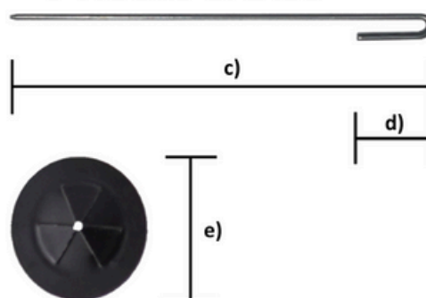
J-Hooks & Disc
