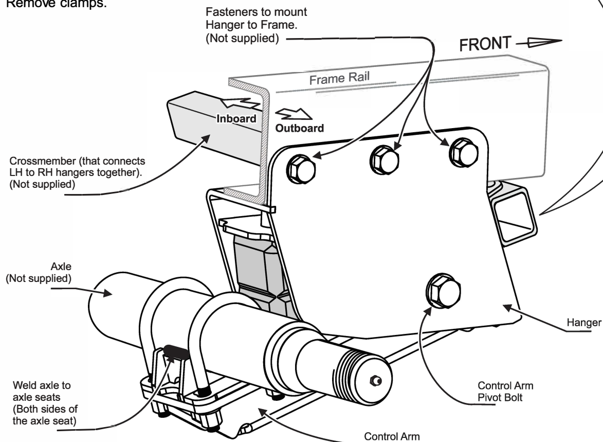
Fig. 2 View of the right-end side suspension on the trailer
