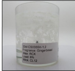
End of Burn Front - Sample 2
