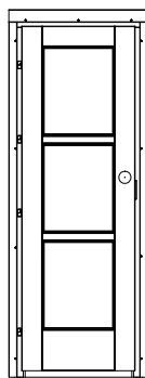
Single Door tempered gl. 1 st. 70 mm 690 x 1955 mm
