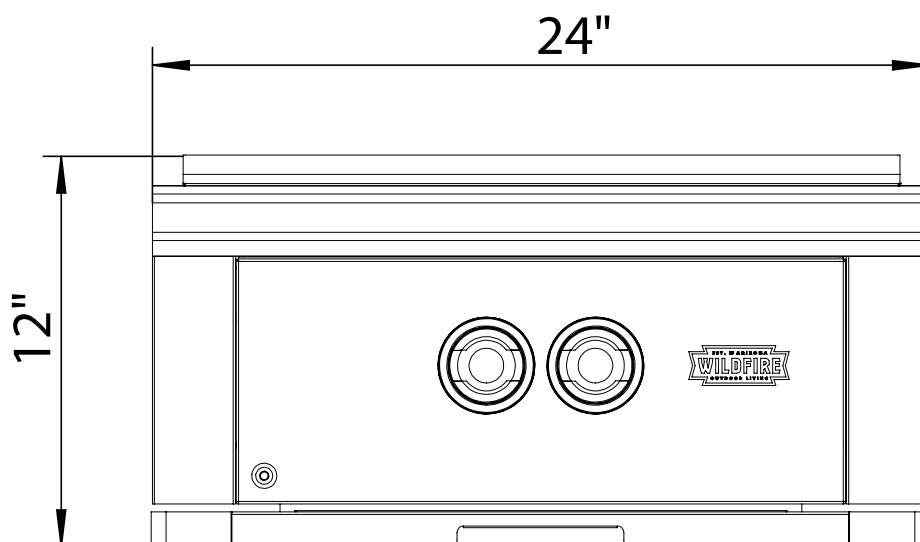
Slide-In Power Burner WF-POWBRN-RH-NG/LG
