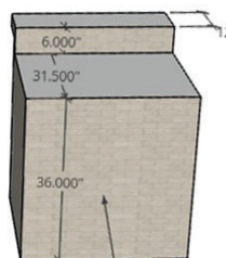
Straight Cabinet With Raised Bar Top
