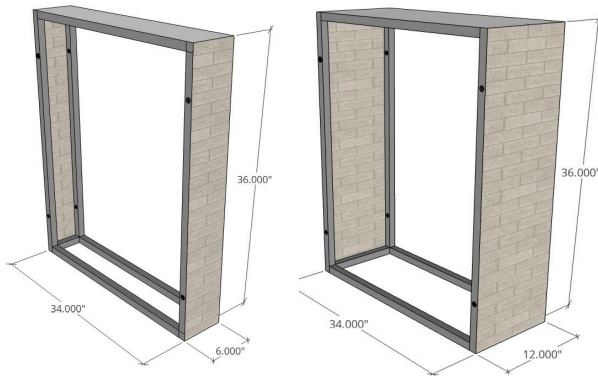
Cabinet, 6" wide - Easy Finish (EZFP6SC)
