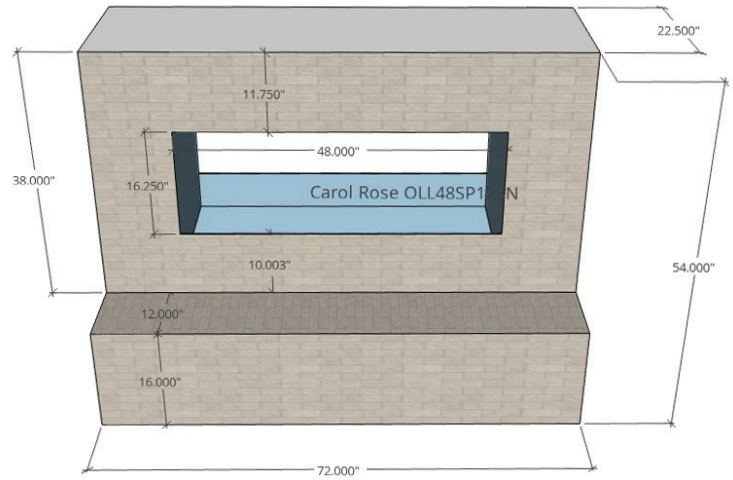
Optional Hearth Two Sided (OFP722S) 12" X 16" X 72"
