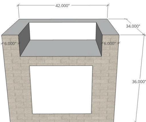
Cabinet, 42" wide - Easy Finish (EZSC42SC) Beverage Center (BLZ-3OCKT-SNK) 25" Access Doors (BLZ-AD25-R)
