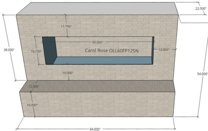
Optional Hearth One Sided (OFP841S) 12" X 16" X 84"
