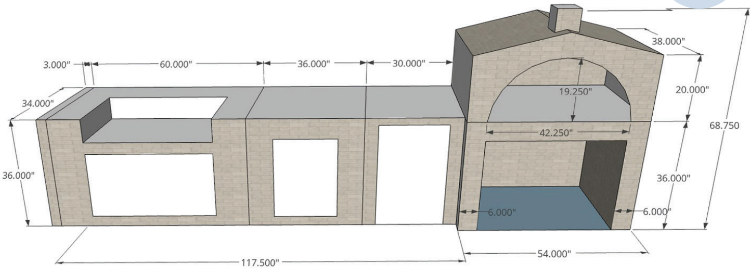
60" Grill Cabinet (EZGC60SC) 36" Trash/Recycling Cabinet (EZTC36SC) • 30" Fridge Cabinet (EZFC3041SC) 60" Pizza Oven Cabinet (EZPO60SC) • 3" End Panel (EXEP3SC) (1)
