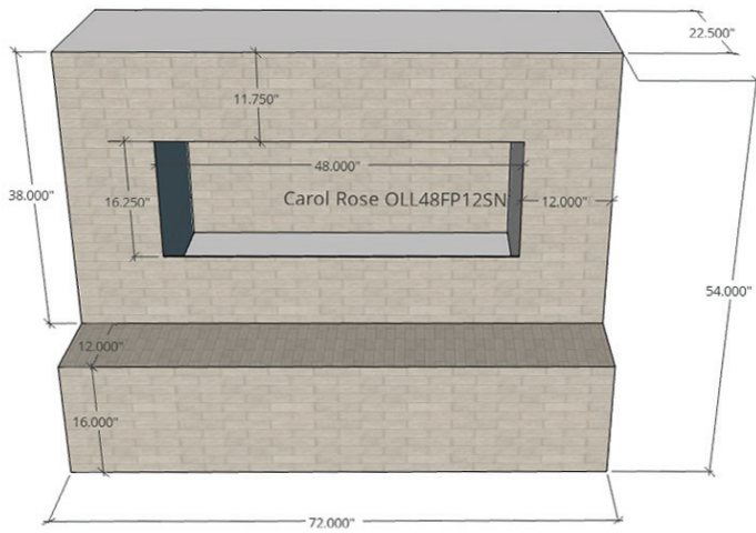
Optional Hearth One Sided (OFP721S) 12" X 16" X 72"
