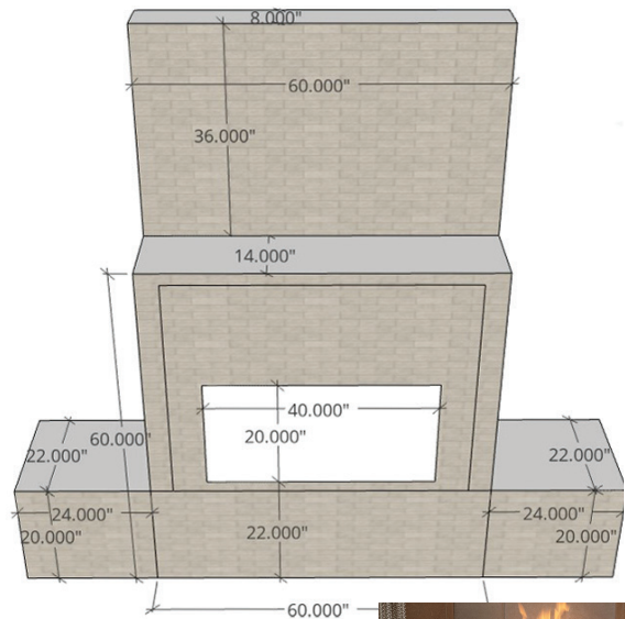
Superior Outdoor Vent-Free Outdoor Fireplace (Model OFP108ST)
