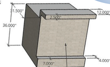
Straight Cabinet With Raised Bar Top
