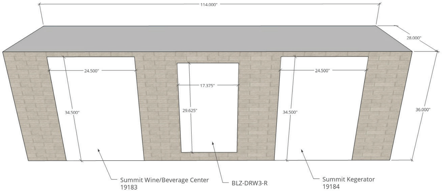
114" Buffet Island (BID114) Bolt on or Stand Alone System Available
