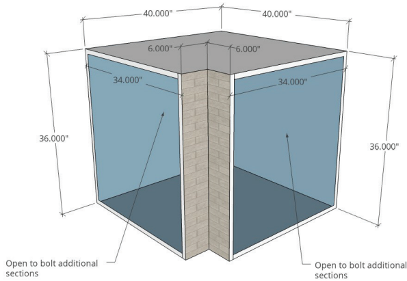
Cabinet, 40"X40" wide - Easy Finish (EZCC4040SC)
