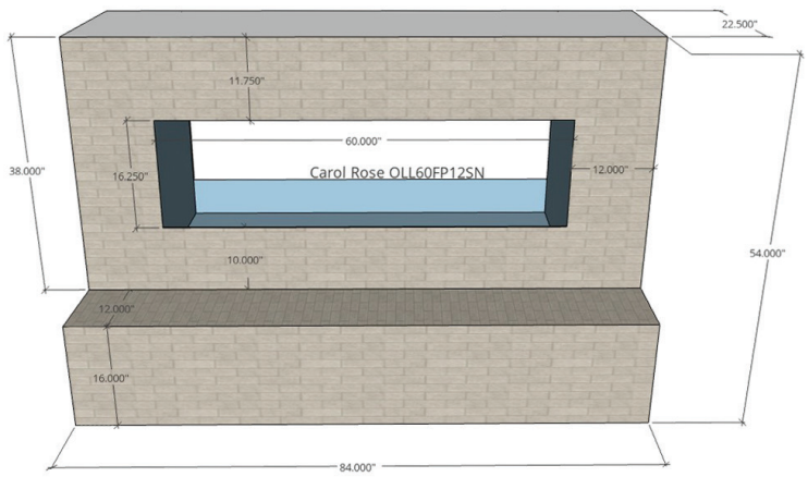
Optional Hearth Two Sided (OFP842S) 12" X 16" X 84"
