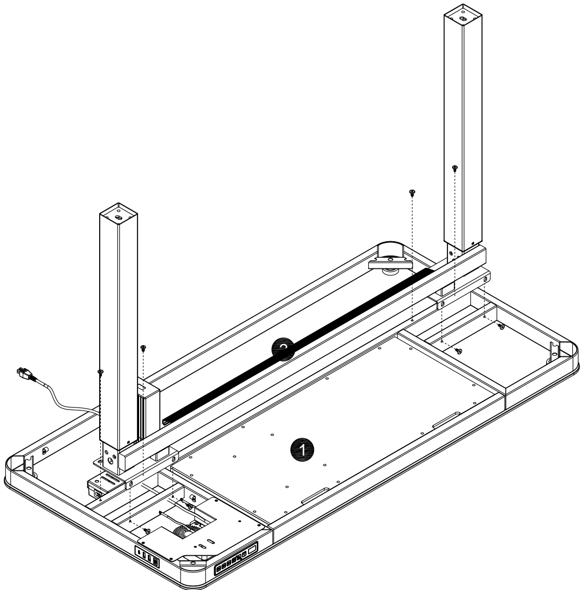
B. 1/2" Small Machine Screw - 8
