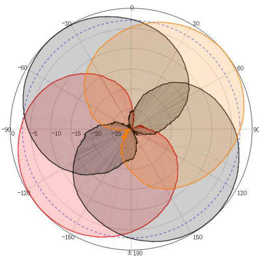
Azimuth patterns
