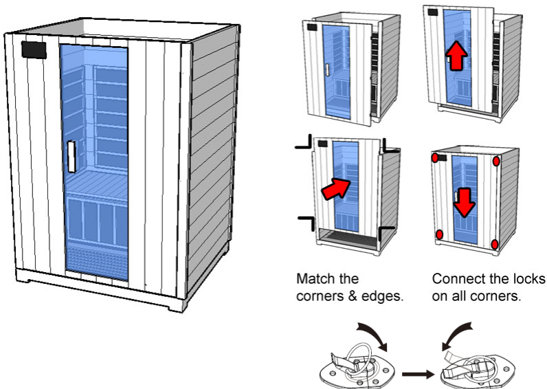
Figure A-5: Front Panel
