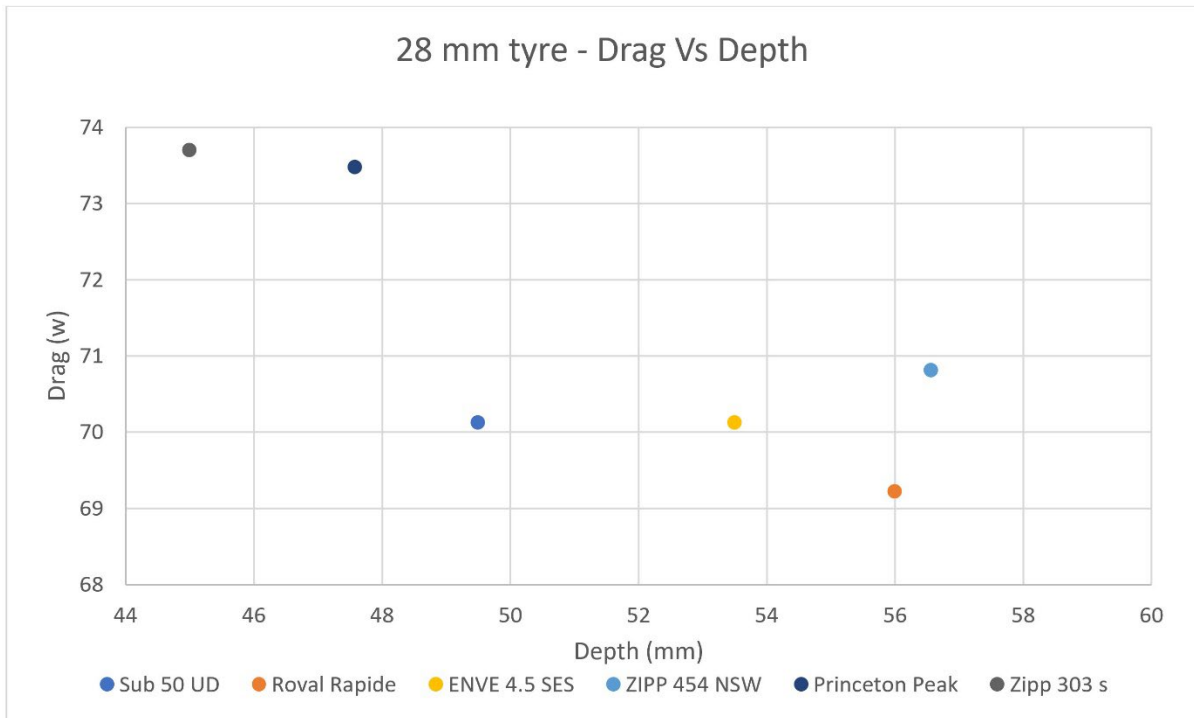
Figure 25 - Drag compared to wheelset depth, with a 28mm tyre.
