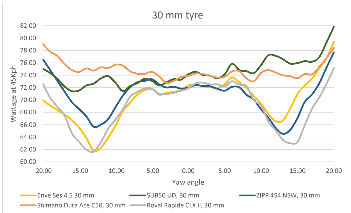
Figure 27 - Results for the key competitor set through -20° to 20°, with a 30mm tyre.
