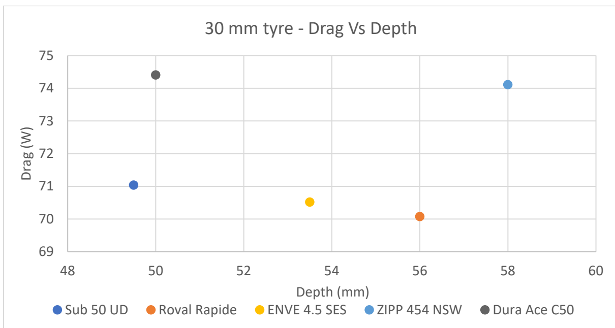
Figure 29 - Drag compared to wheelset depth, with a 30mm tyre.
