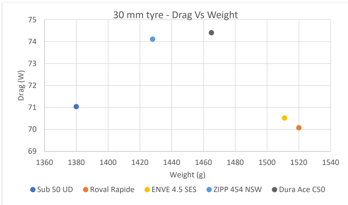
Figure 28 - Drag compared to wheelset claimed weight, with a 30mm tyre
