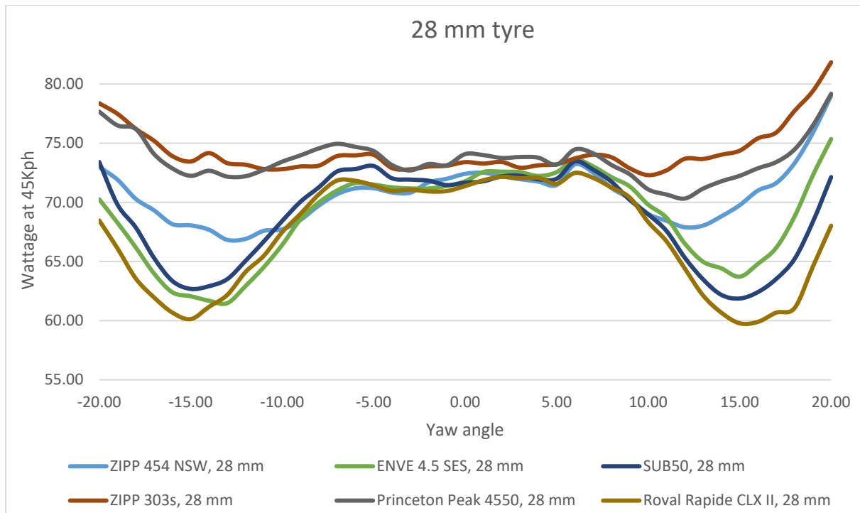
Figure 23 - Results for the key competitor set through -20^{\circ} to 20^{\circ} , with a 28mm tyre.
