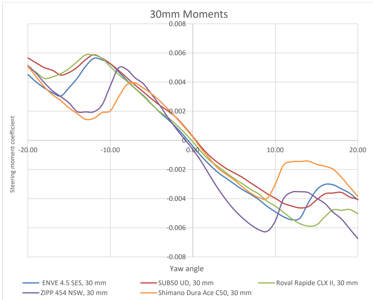
Figure 30 - Graph showing the steering moment coefficient with a 30mm tyre through -20^{\circ} to 20^{\circ} .
