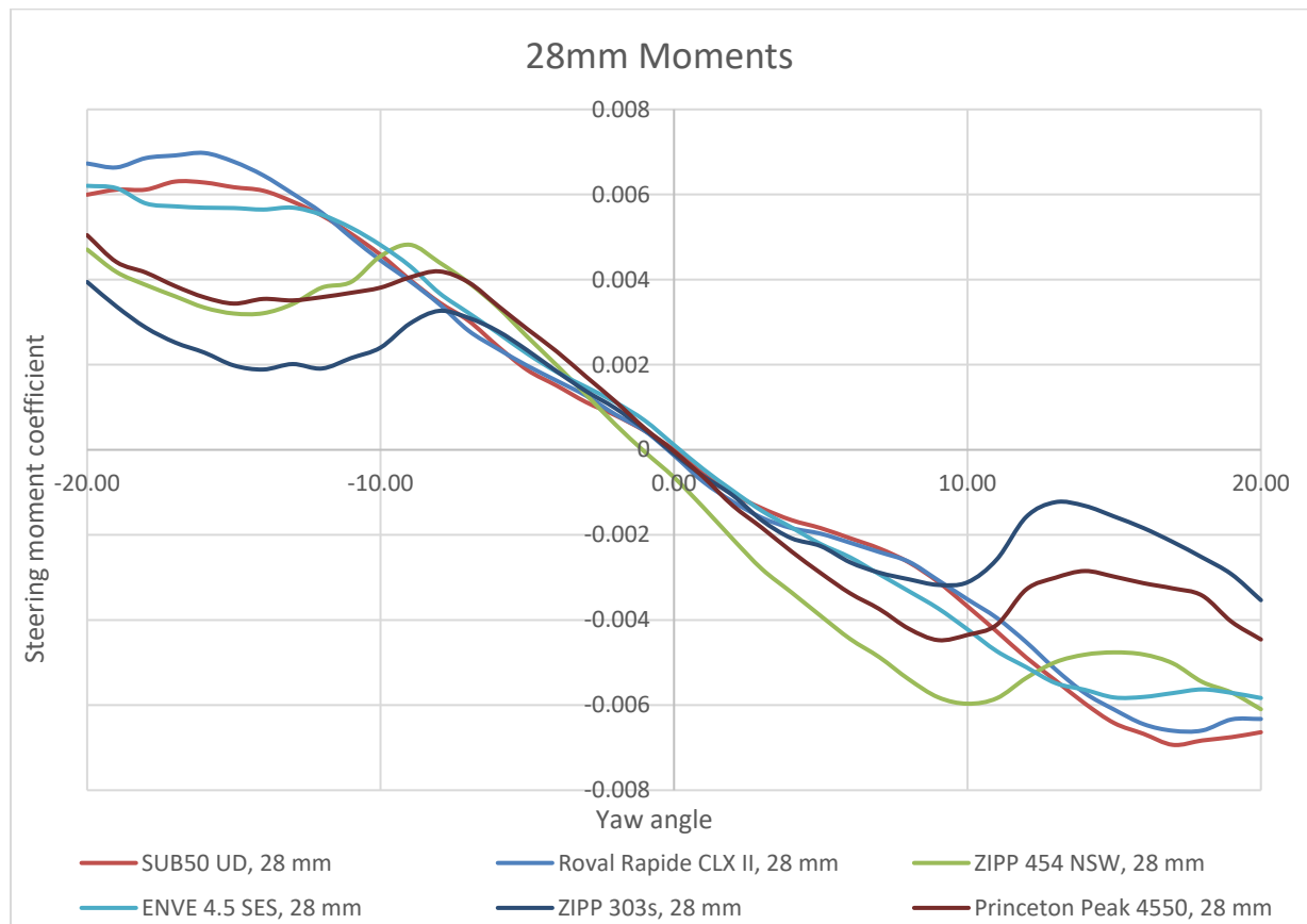
Figure 26 - Graph showing the steering moment coefficient with a 28mm tyre through -20^{\circ} to 20^{\circ} .
