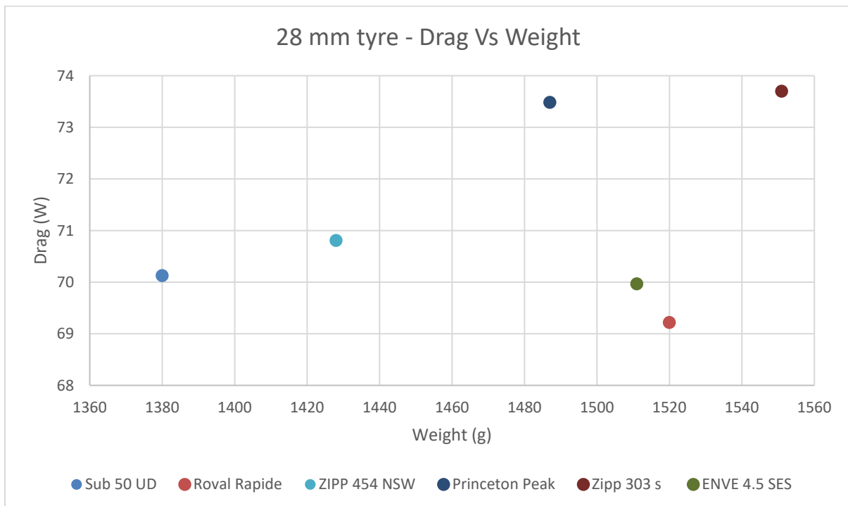
Figure 25 - Drag compared to wheelset claimed weight, with a 28mm tyre.
