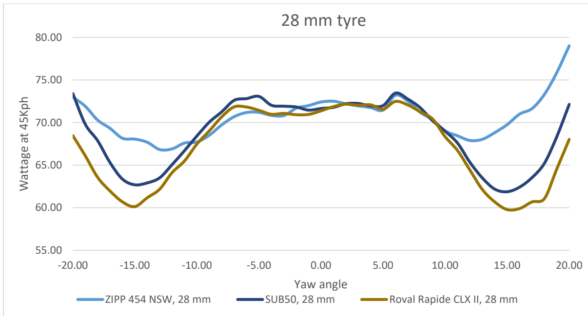
Figure 24 - Results for the fastest wheels through -20^{\circ} to 20^{\circ} , with a 28mm tyre.
