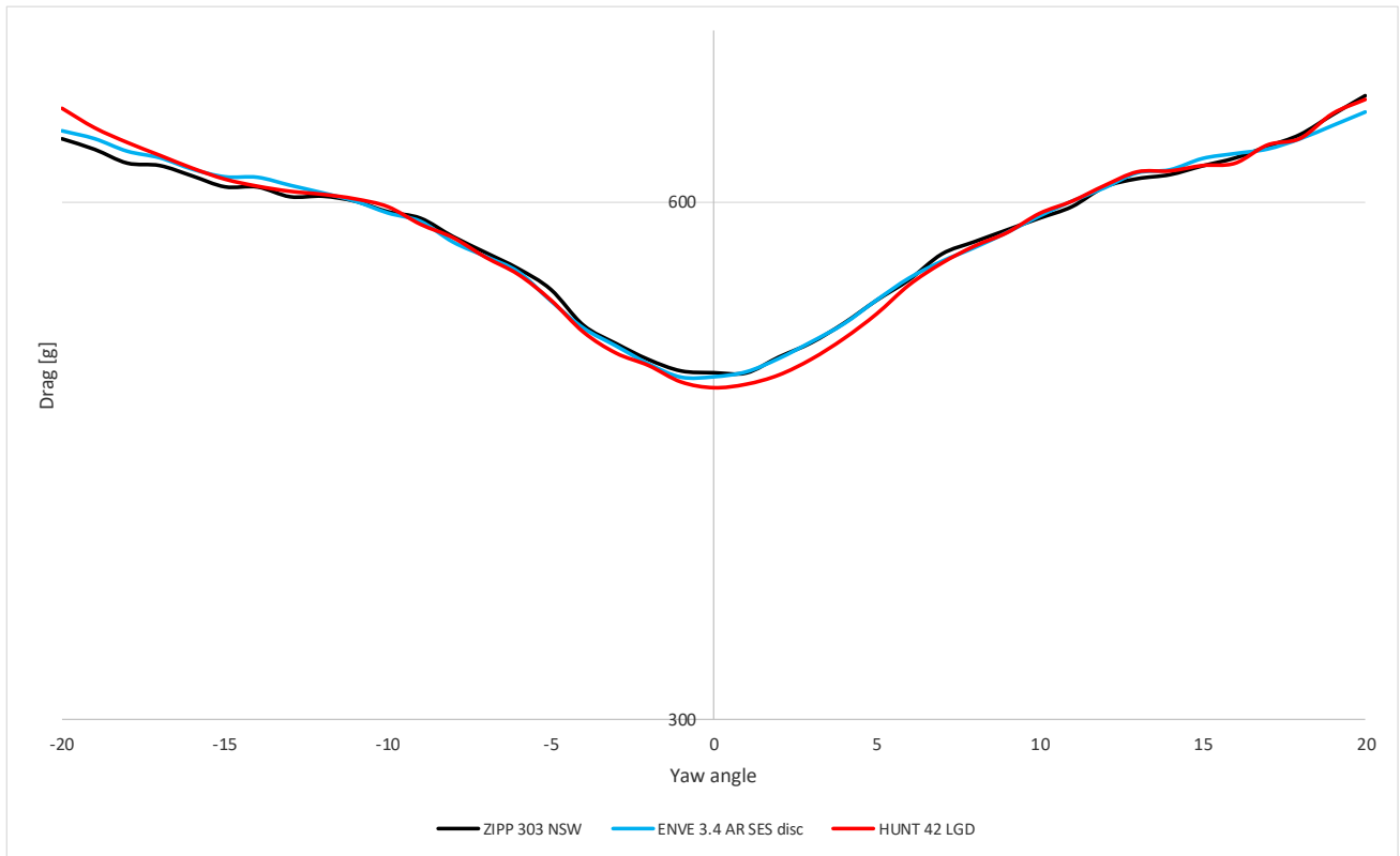
Figure 5: Drag [g] vs yaw angle [°] from wind tunnel test showing HUNT 42 LIMITLESS GRAVEL DISC against competitors, using a Terravail Cannonball 42mm tyre at 32km/h
