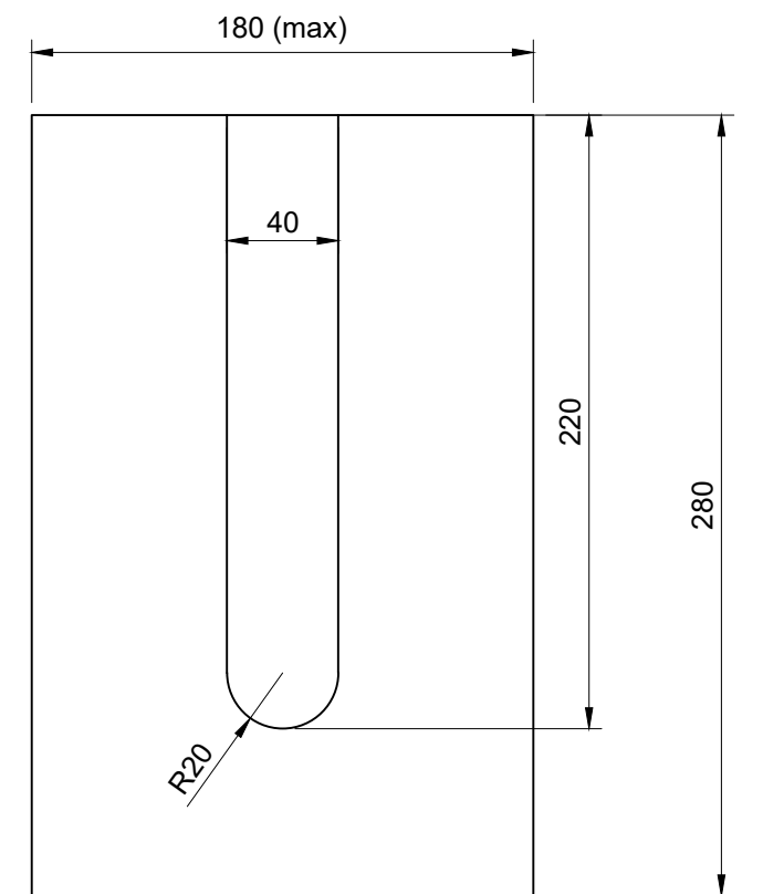
LTZ40 Dimensions
