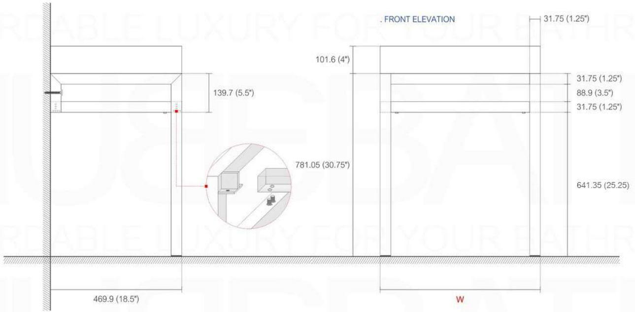
. SIDE ELEVATION
