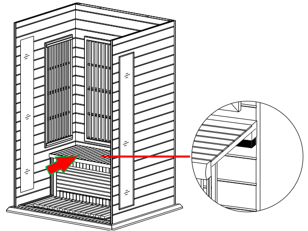
FIG 10 Installing Bench
