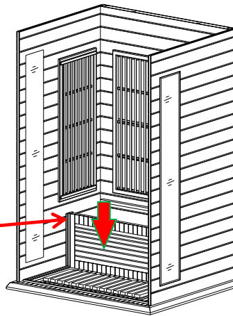
FIG 9 Installing Bench Heat Emitter
