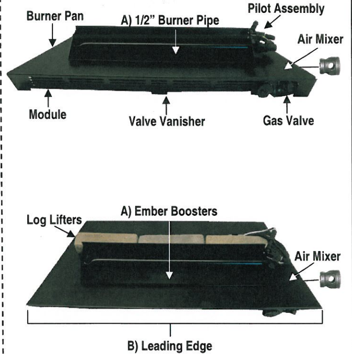
FIGURE 7 Propane
