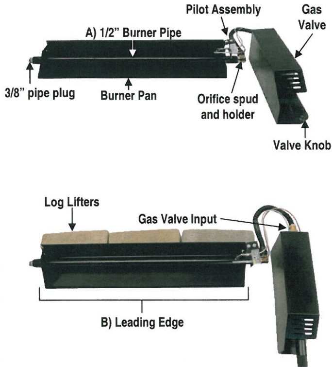
FIGURE 6 Natural Gas
