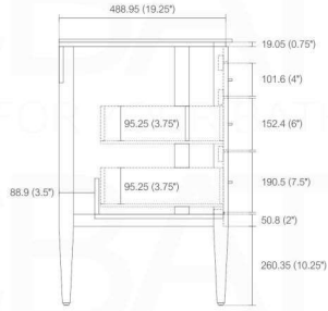
SIDE ELEVATION
