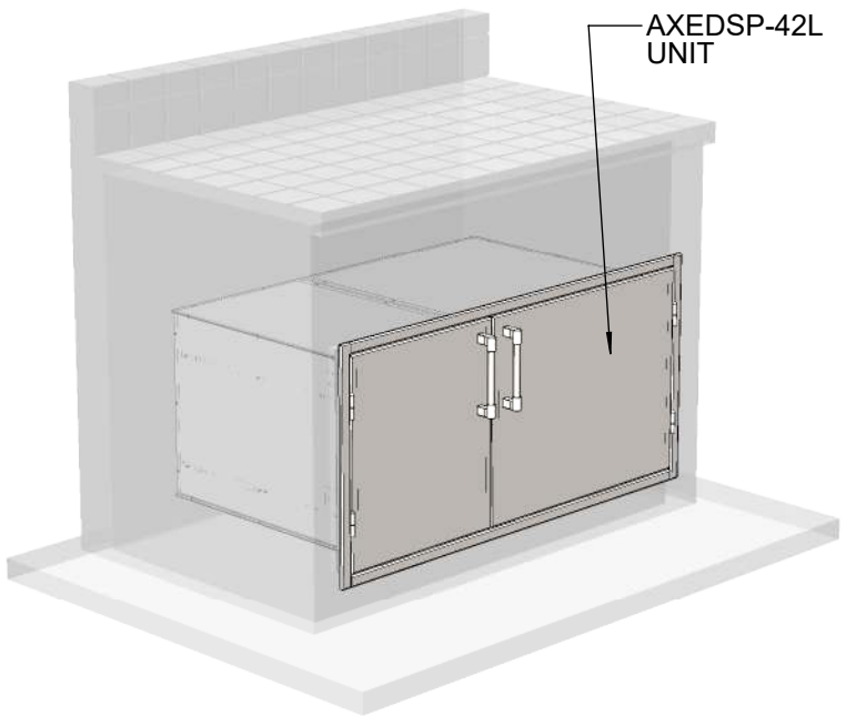
AXEDSP-42L TYPICAL INSTALLATION
