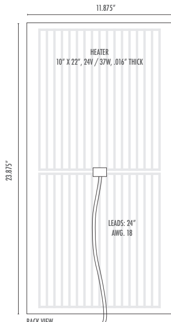
BACK VIEW SCALE 3"=1'-0"
