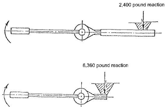
Figure 1 Reaction forces increase the closer the reaction point is to the multiplier.
