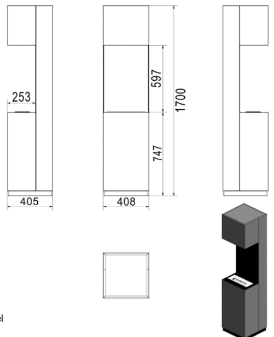
Weight: 48.5kg Material: black or white MDF, painted steel Optional: glass protection screen
