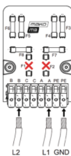
1-Phase Power Input L-L = 208-480 Vac
